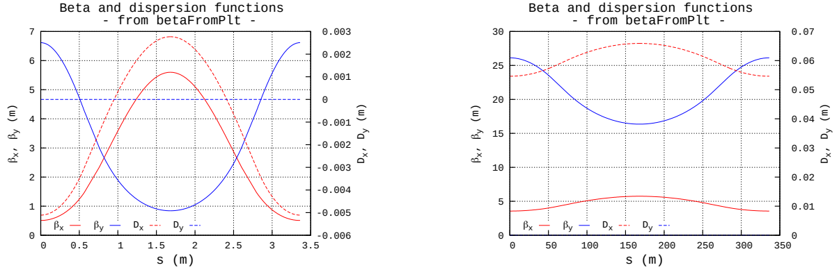
Figure 5: Optical functions at 6.622 GeV (left) and 21.164 GeV (right) from stepwise ray-tracing across the FFA cell.
