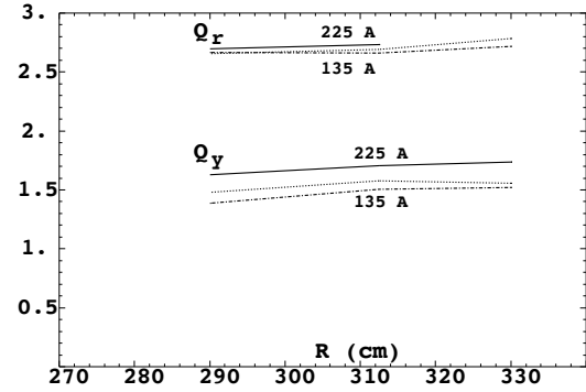
(b) Vertical tune Q_y derived from measured fields at 135, 180 and 225 A. At 225 A the measured field is 1.933 T at R=3.46 m.
