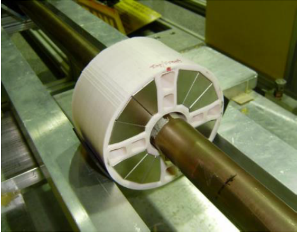
Figure 8: A modified Halbach quadrupole to avoid the synchrotron radiation, and a rotating coil device which measures the integrated multipoles of the magnet. The white material of the magnet is to hold the permanent magnet wedges together for the magnetic measurements only. The actual assembly of the magnet is different.
