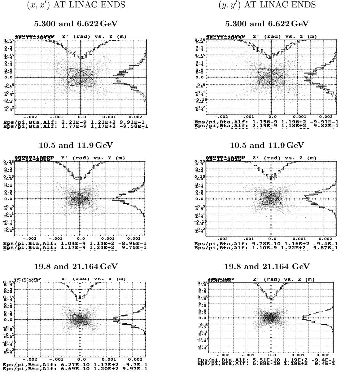
Figure 18: Bunch transverse emittances (non-normalized) and \beta_x, \alpha_x, \beta_y, \alpha_y parameters are given below the plots for each energy. These parameters appear to be well preserved, with \beta\gamma betatron damping as expected, i.e. the same normalized emittances at the linac entrance and exit.
