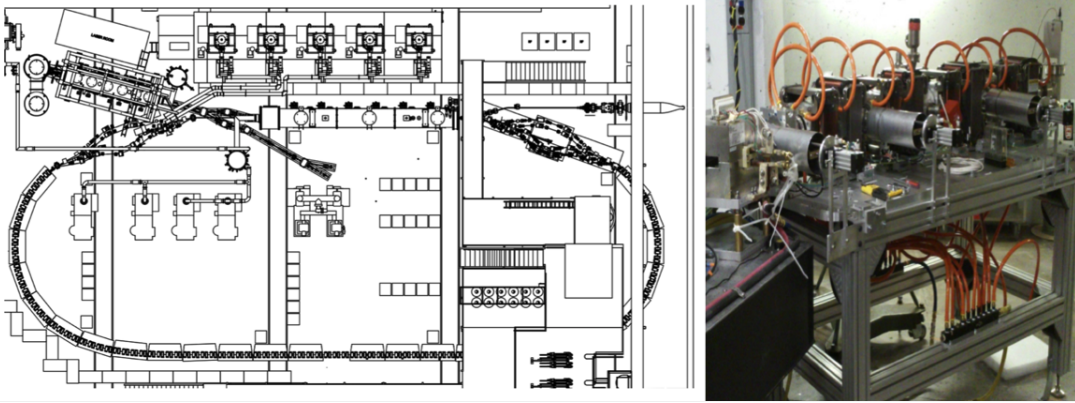
Figure 1: The CBETA layout (left) and first magnet girder (right) where the permanent halfbach magnets are small magnets close to the beam pipe, embedded within the more visible corrector coils.
