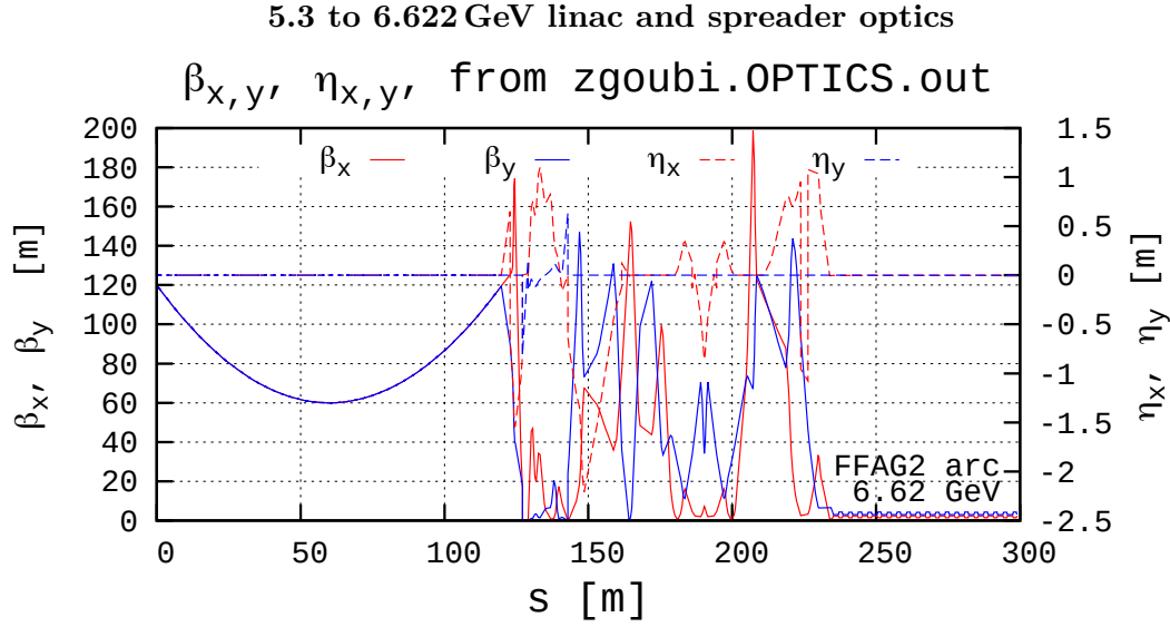
Figure 15: Details of the optical functions (betatron, left axis, and dispersion, right axis), in the case of the 5.3 \rightarrow 6.622 GeV linac energy step. The \beta_x, \beta_y parabolas on the left correspond to the linac (120 m long). The linac is followed by a spreader line which ends up steering the beam on its 6.622 GeV orbit in the FFA loop on the way up. The FFA loop extends into the s > 230 m region (to the right), with betatron amplitudes \beta_x, \beta_y = 5.6, 6.6 m and dispersion function amplitude -5 to +3 mm (see Fig. 5). The latter features \sim \pm 1.5 m excursion in the spreader.
