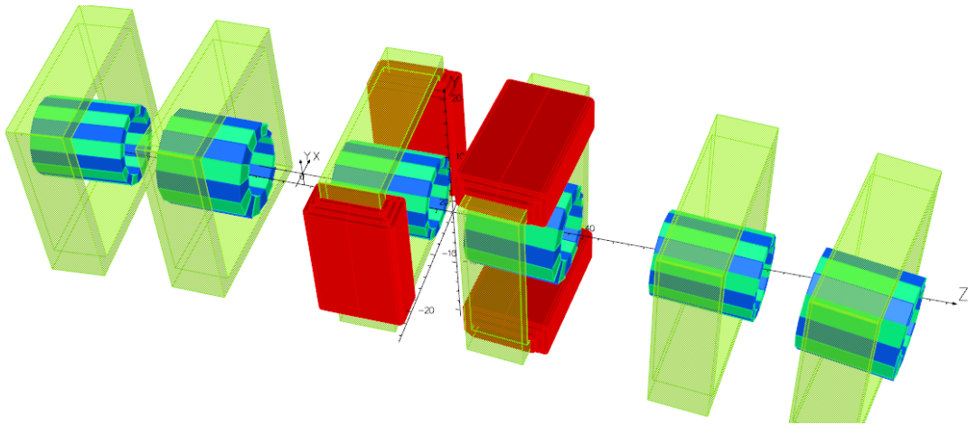
Figure 2: A perspective view of three consecutive cells of the (FA) or (FB) sections of the FFA transfer line shown in Fig. 1. Each cell consists of a focusing pure quadrupole (QF) and a combined function magnet (BD) providing a dipole and defocusing quadrupole. Both magnets QF and BD are Halbach type magnets and each magnet has a dipole corrector window frame magnet which surrounds the magnet. The dipole corrector of the QF magnet generates vertical field and that of the BD generates horizontal field.
