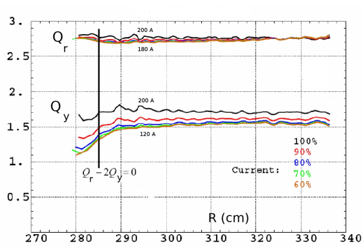
(a) Horizontal tune Q_r derived from OPERA data, with currents in the 120-200 A range. At 200 A the OPERA model field is 1.7 T at R=3.46 m.
