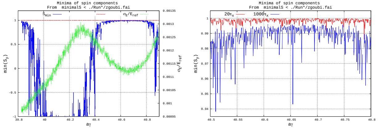
Figure 9: An ergodic approach to polarization lifetime in the 18 GeV eRHIC electron storage ring. Left, blue curve: depolarization landscape S_{y,min}(a\gamma_{ref})|_{t \in [0,T]} (the smallest value reached by the vertical spin component over the tracking interval [0, T] ) over 39.8 < a\gamma_{ref} < 40.9 (200 bins of \Delta E = 0.44 MeV, a single particle per bin), after T \approx several thousand turns tracking. The right vertical scale (green curve) is the rms width of the energy interval explored by a particle during the tracking. Right: a zoom in on a reduced 40.5 < a\gamma_{ref} < 40.8 interval, showing S_{y,min}(a\gamma_{ref})|_{t \in [0,T]} at (red) 9500 turns and (blue) 450,000 turns (6 s storage).
